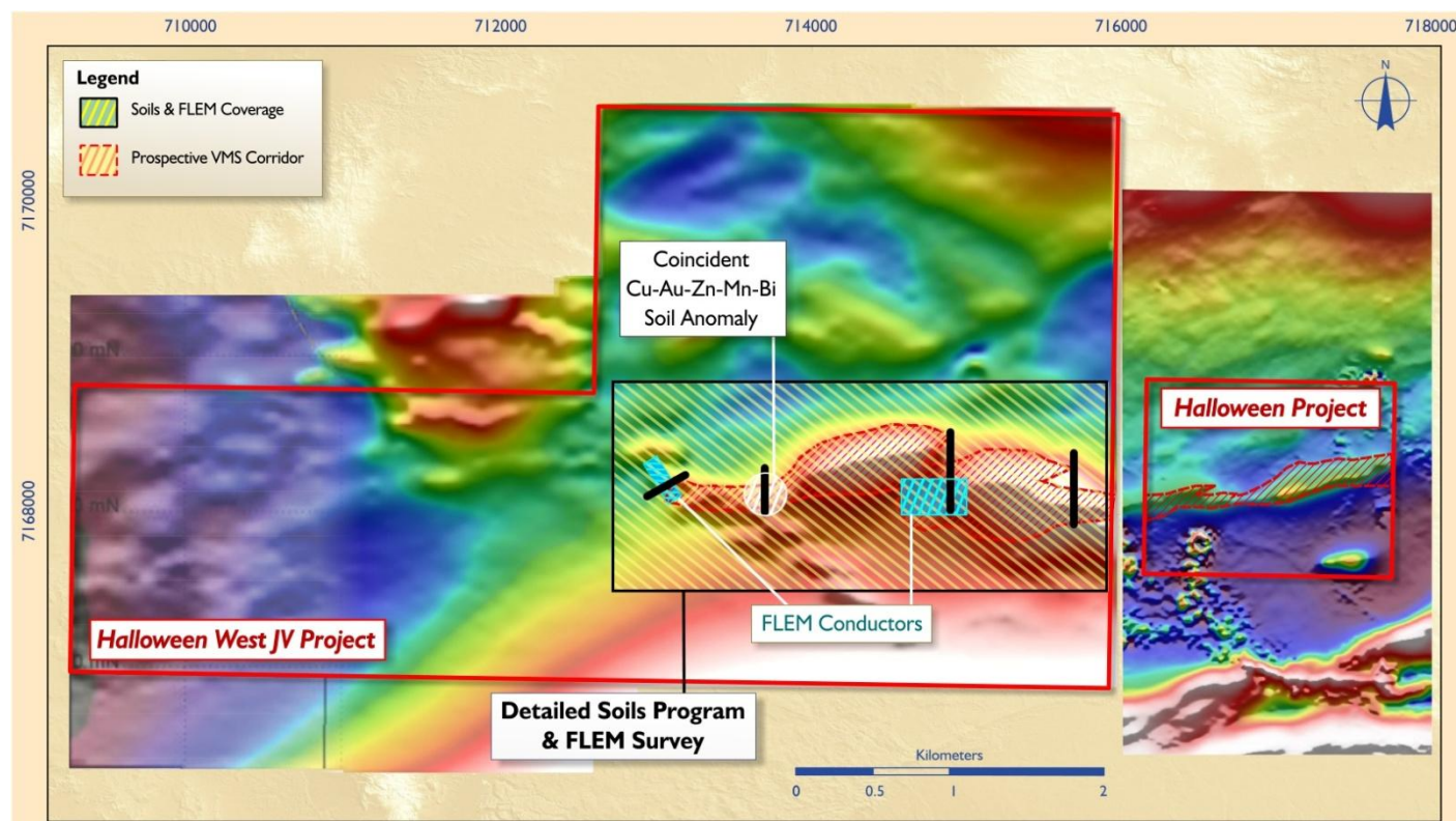
Figure 2 – Halloween West JV Project showing geochemical and electromagnetic targets and proposed drill traverses along the prospective Halloween VMS Horizon
