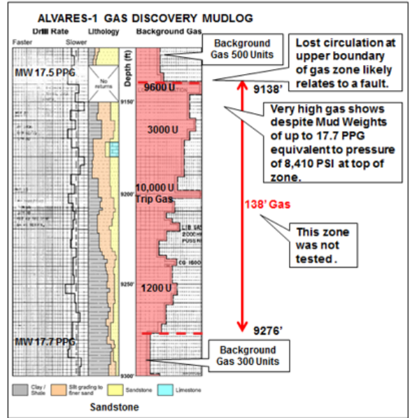
Untested Gas Zone in Alvares-1
