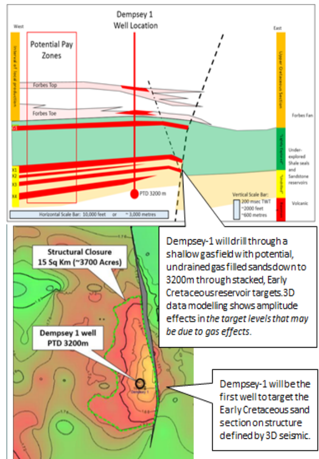
Cross section and Map of Dempsey Gas Project
